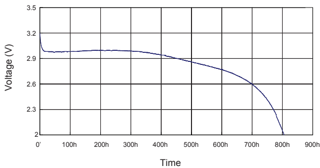
2mA continuous discharge to 2.0V at 23°C
