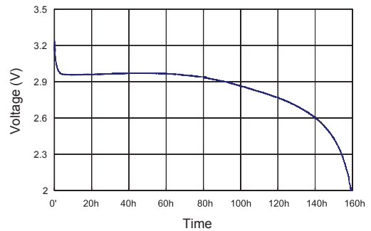
10mA continuous discharge to 2.0V at 23°C
