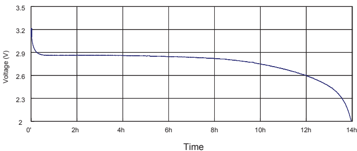
100mA continuous discharge to 2.0V at 23°C
