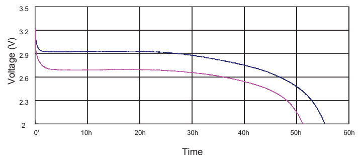
100Ω continuous discharge to 2.0V at 23°C & -20°C
